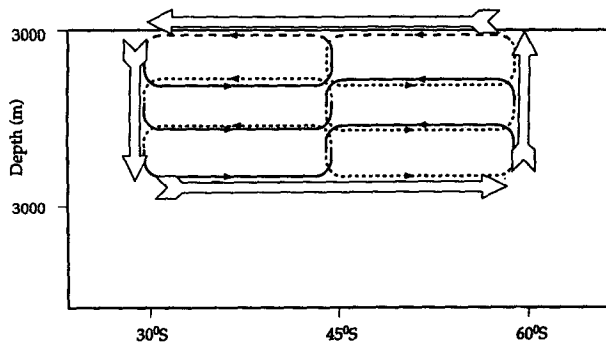
FIG. 9. A schematic view of the Deacon cell. The cells represent the circulation on isopycnals in the subtropical gyres to the north, and in the Antarctic Circumpolar Current to the south. The solid lines represent flows in the western boundary current region off South America, dashed lines represent flows in the rest of the ocean, and long dashes flows in the surface Ekman layer. The large arrows represent the Deacon cell, which results from integrating the flows zonally on depth levels.
