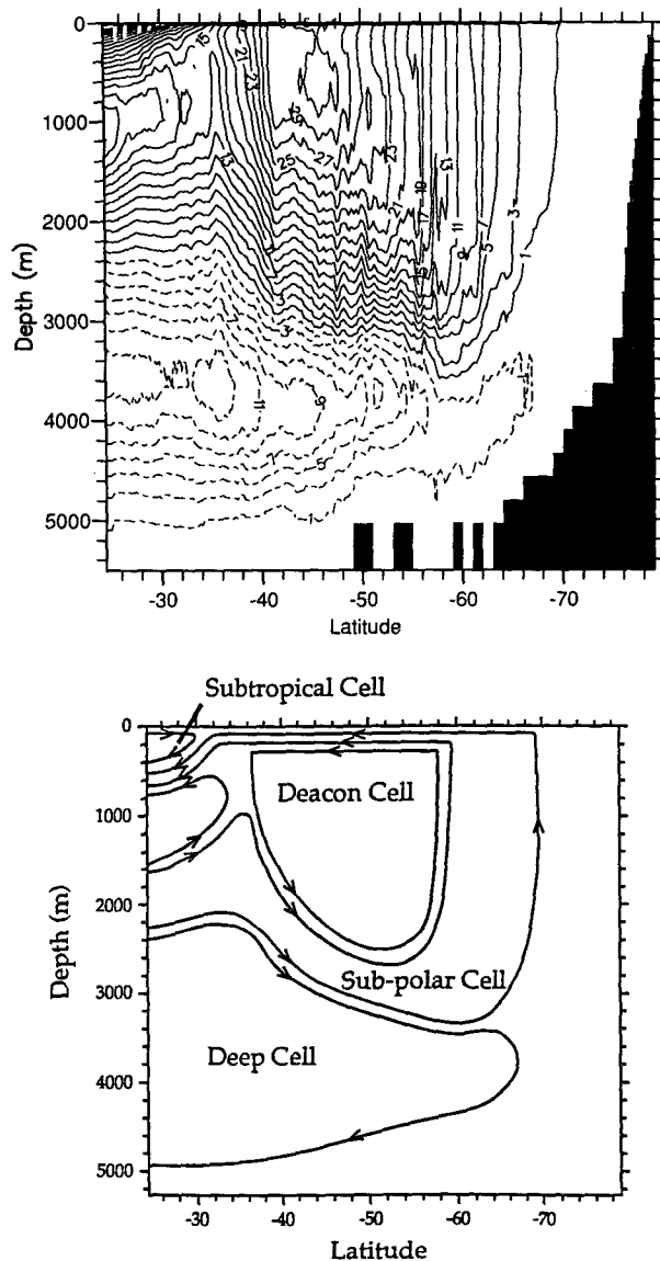
FIG. 2. (a) The meridional streamfunction from the FRAM model, where the zonal integration has been carried out at fixed depths. Units are in Sverdrups ( 1 \text{ Sv} = 10^6 \text{ m}^3 \text{ s}^{-1} ). (b) Schematic showing the names and direction of flow of the different cells.
