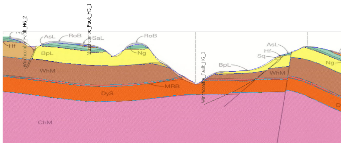
Figure 6 - Moreton-In-Marsh 1:50,000 scale map image as a backdrop in GSI3D cross-section
