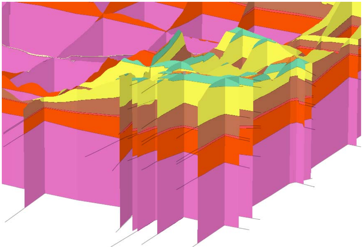
Figure 8 - Correlated cross-sections in 3D (x5 vertical exaggeration)
